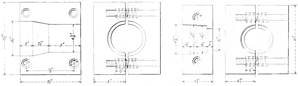
Dies for Swedging Superheater Flues
